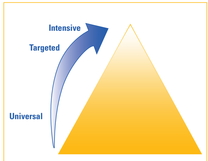
Figure 1: SWPBIS Model
